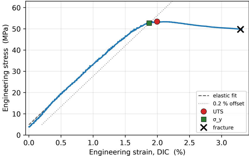
Stress-strain
